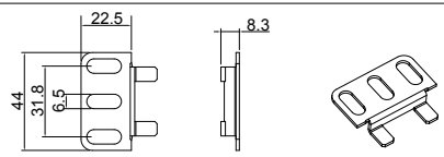
Mounting Bracket
